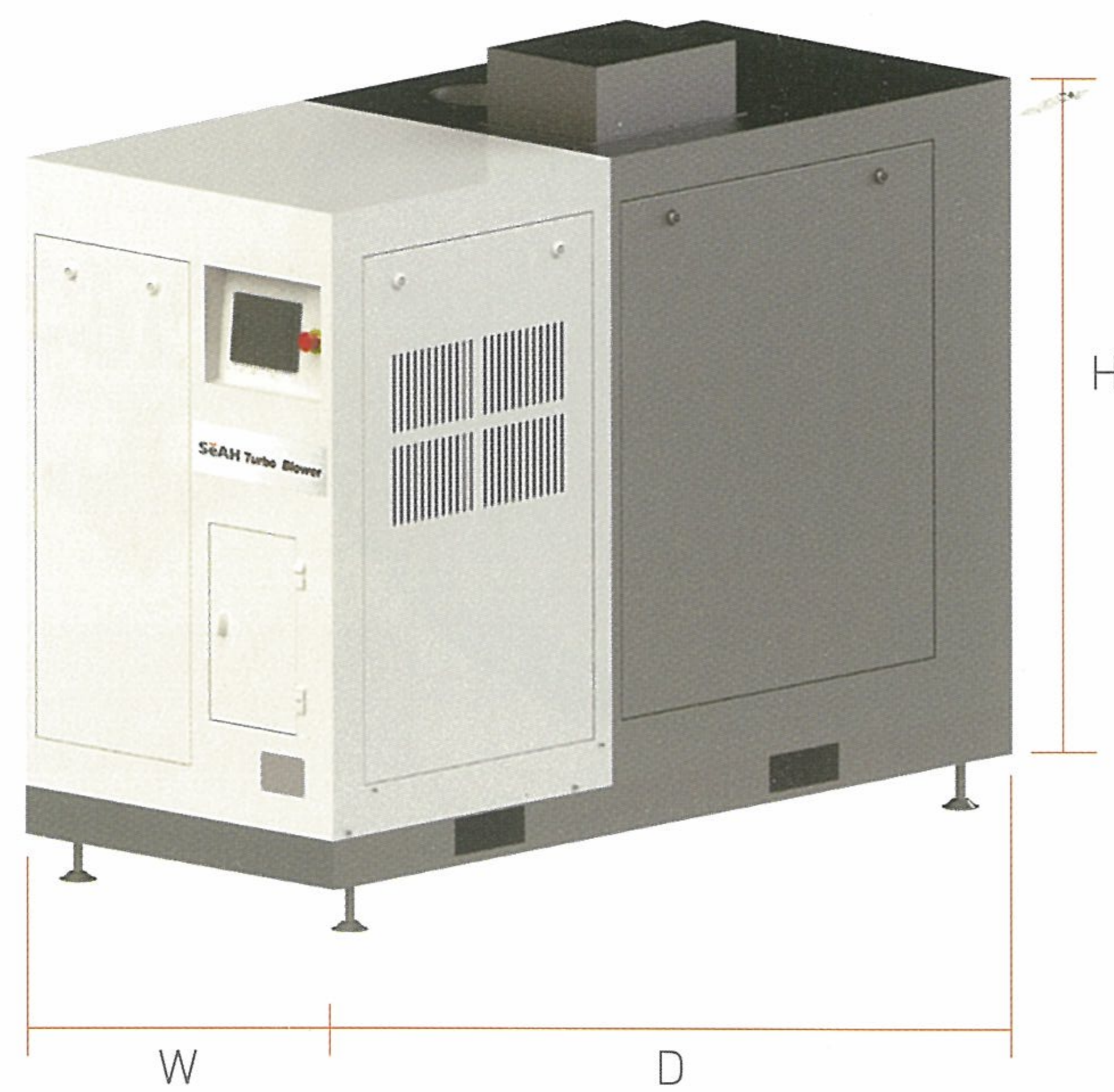
Front View
